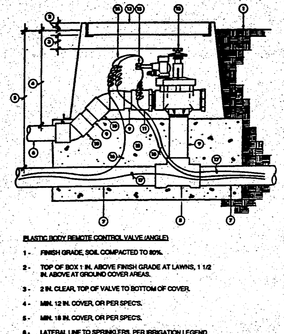
REMOTE CONTROL VALVE
