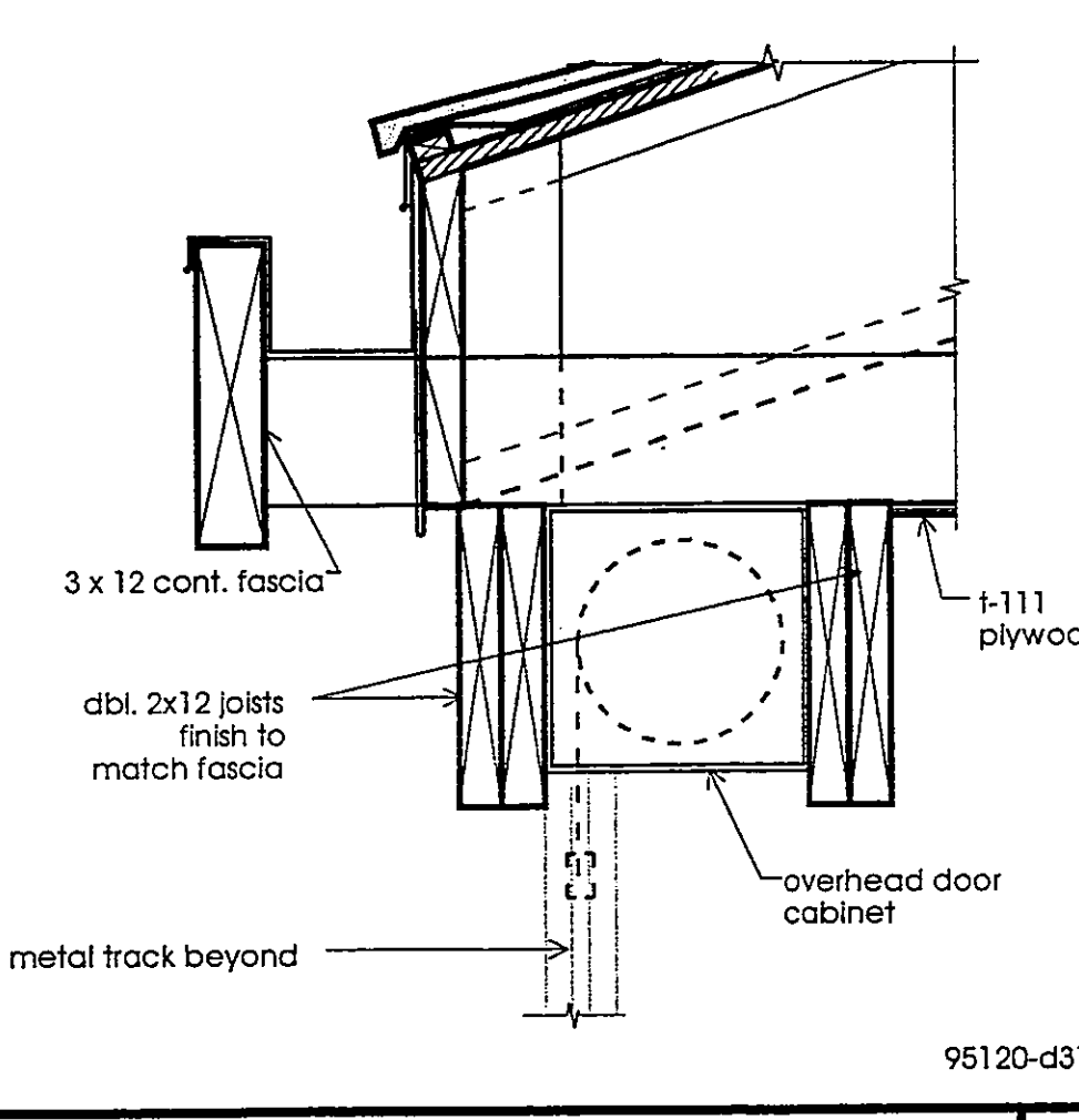
OVERHEAD DOOR 1 1/2" = 1'-0" 10
