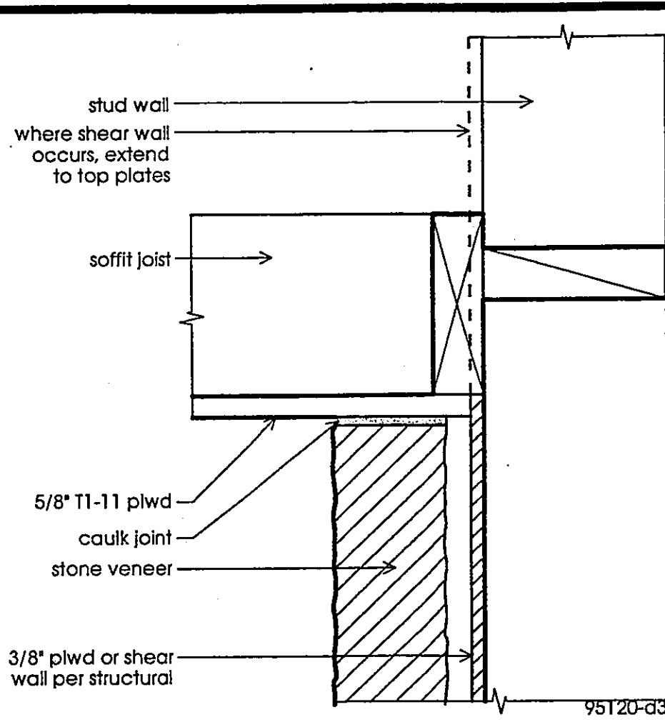
SOFFIT AT VENEER Scale: 3" = 1'-0" 2
