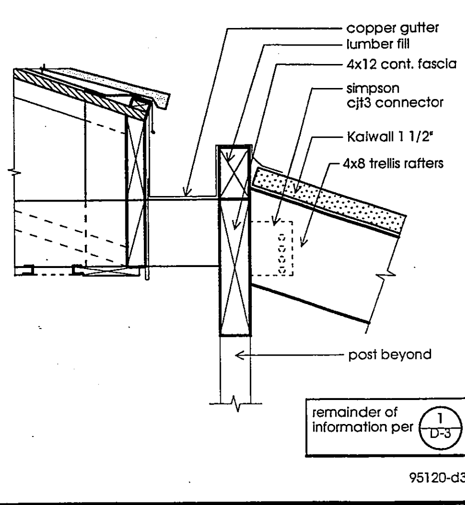
EAVE AT TRELLIS Scale: 1 1/2" = 1'-0" 9
