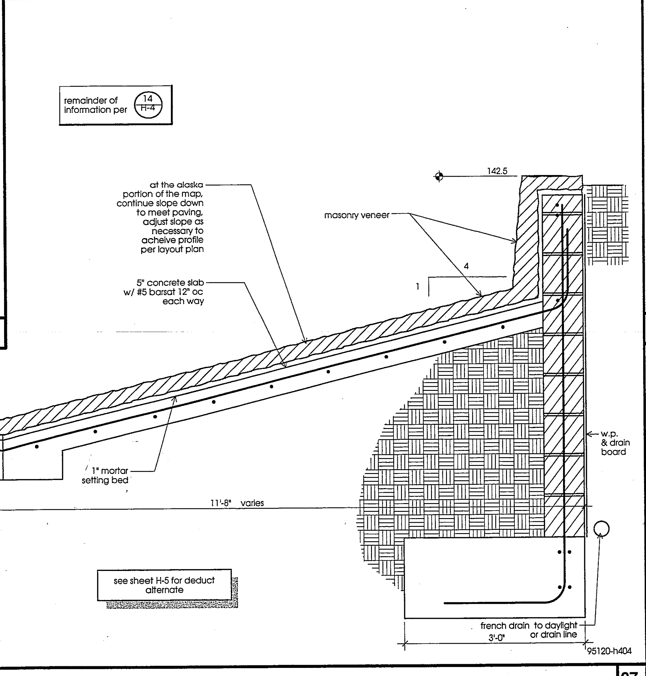
TERRACE STAIR
