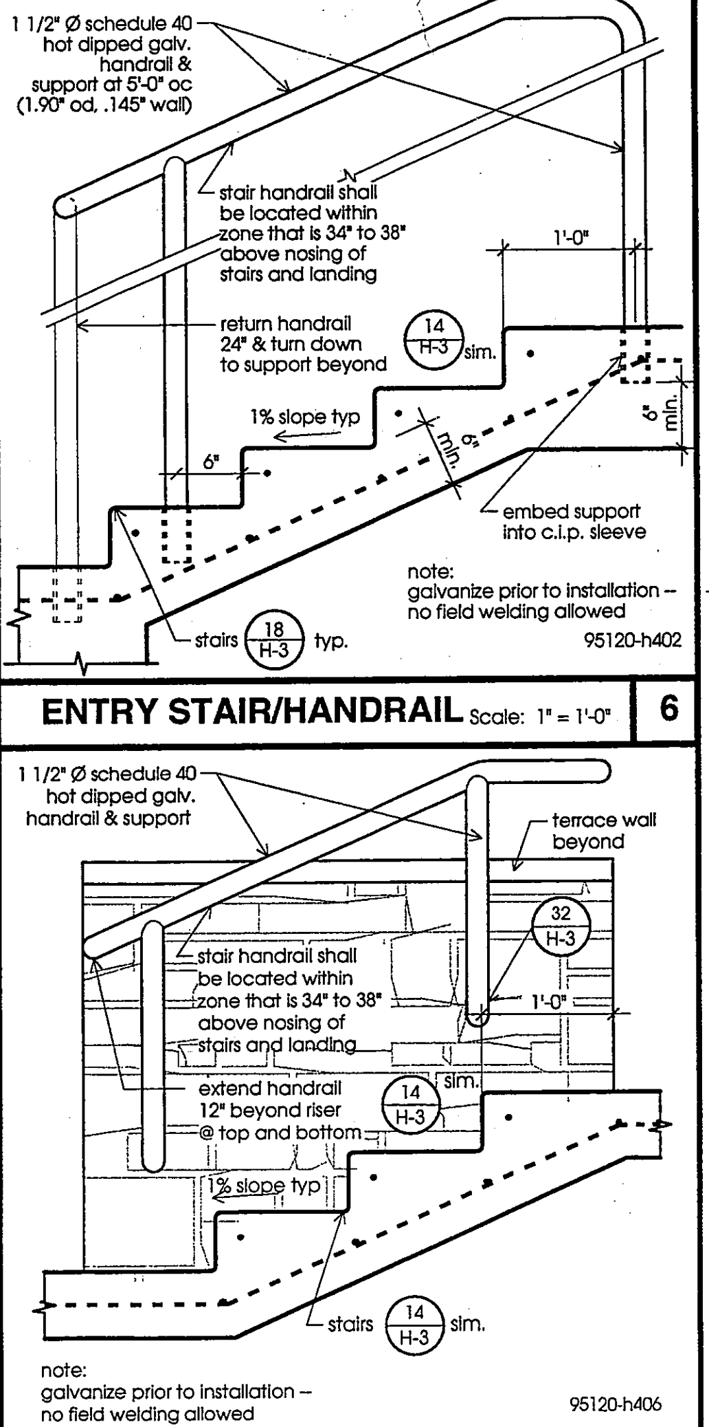
ENTRY STAIR/HANDRAIL
