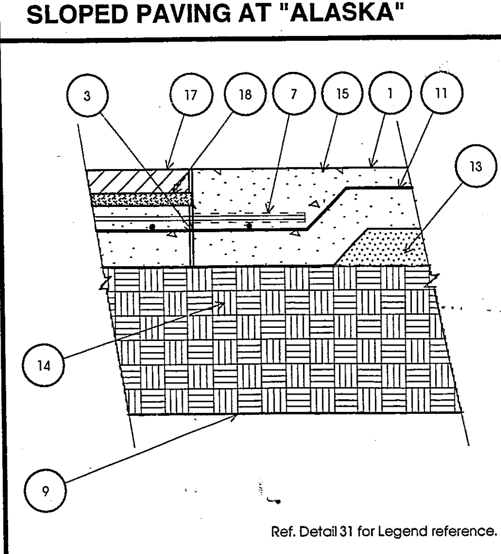
SLOPED PAVING AT "ALASKA"
