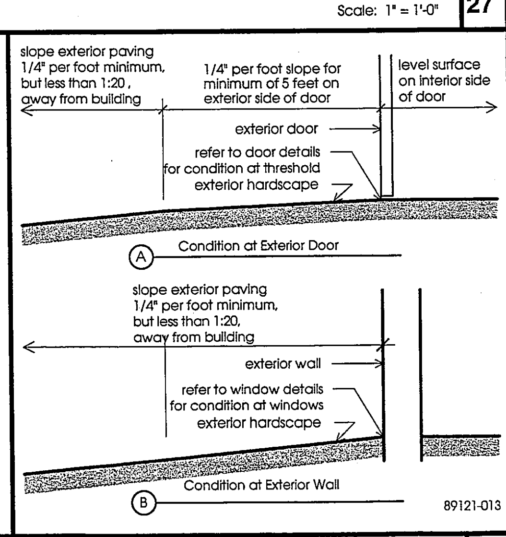
HARDSCAPE @ BLDG.
