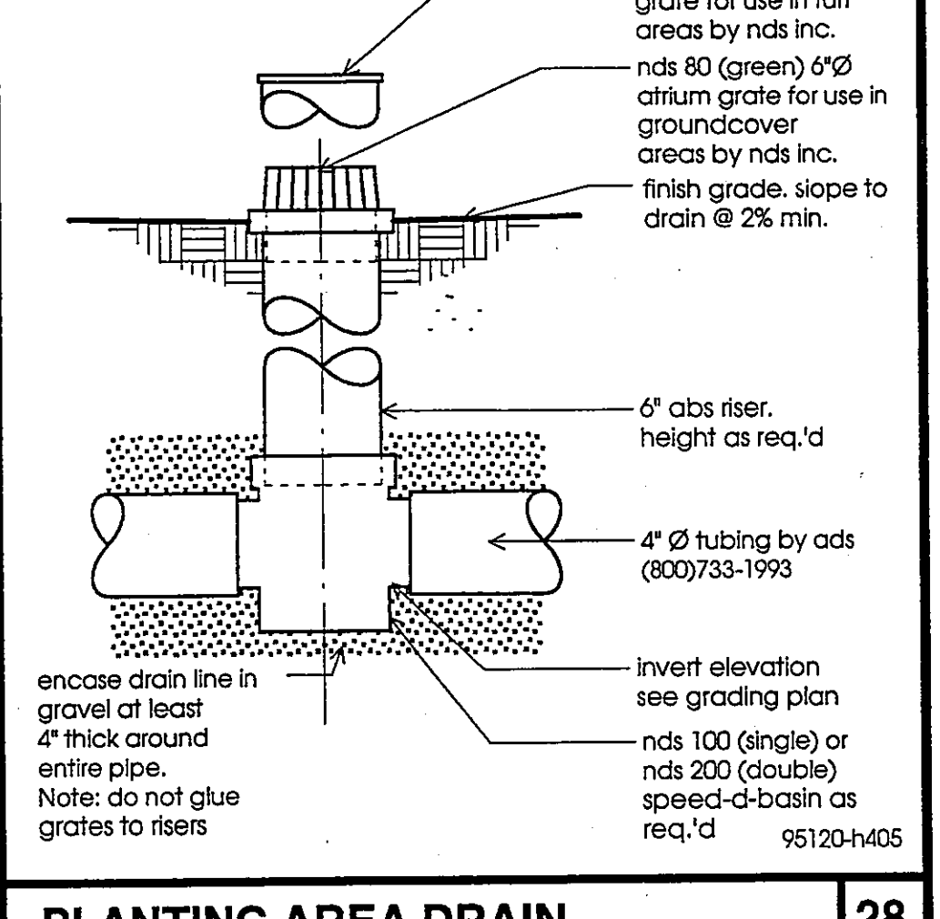
PLANTING AREA DRAIN
