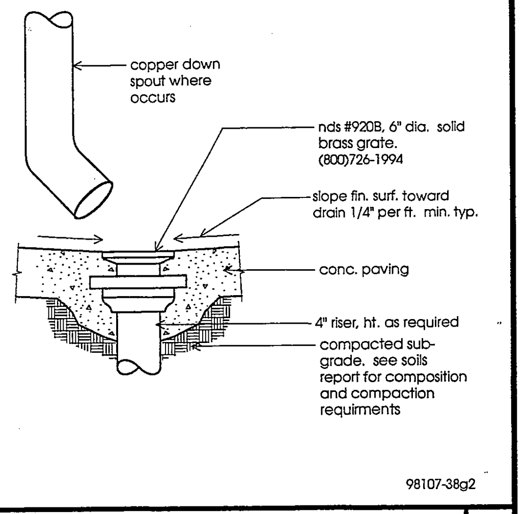
PAVING AREA DRAIN
