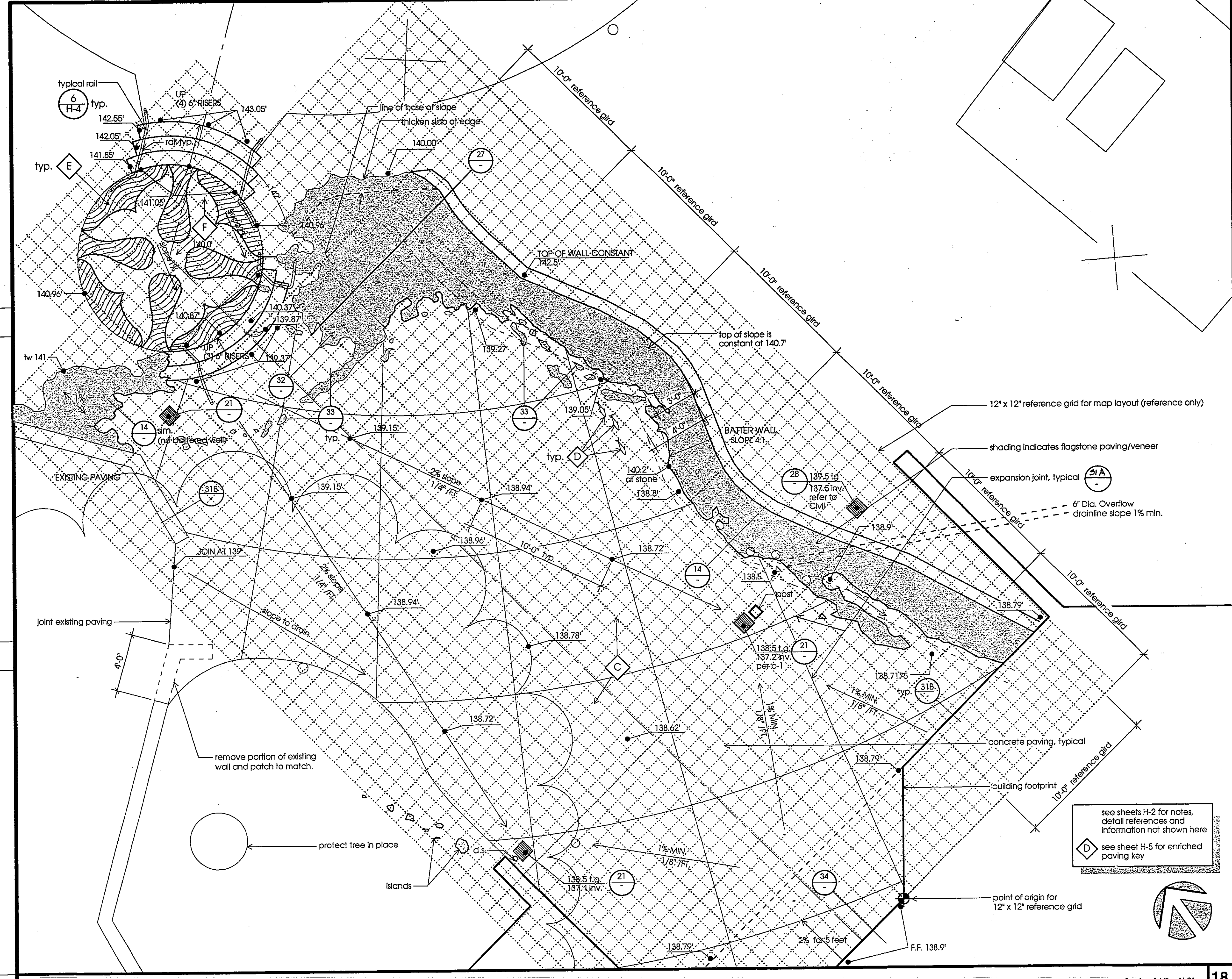
STONE PAVING MAP LAYOUT PLAN
