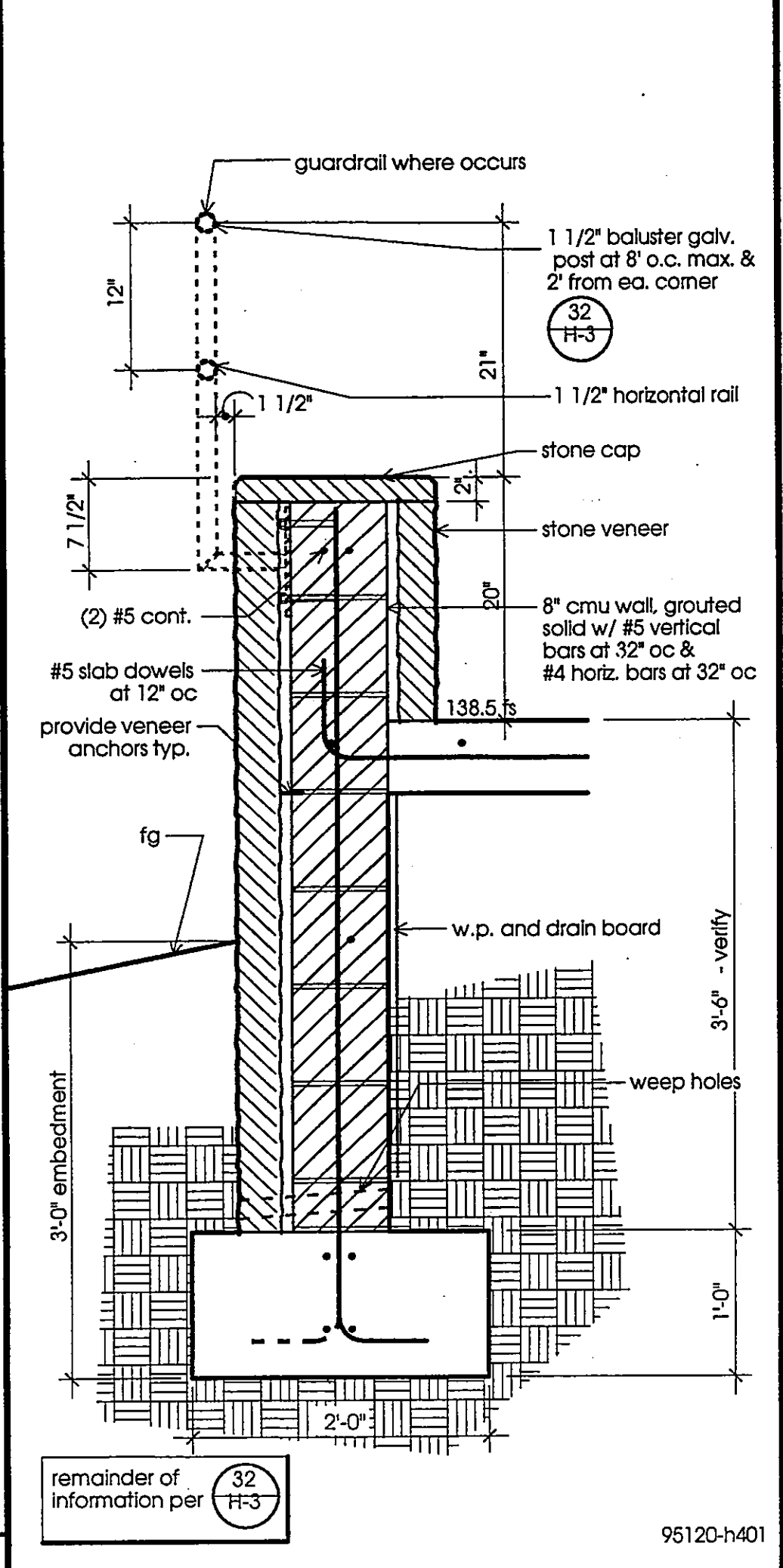
TERRACE WALL
