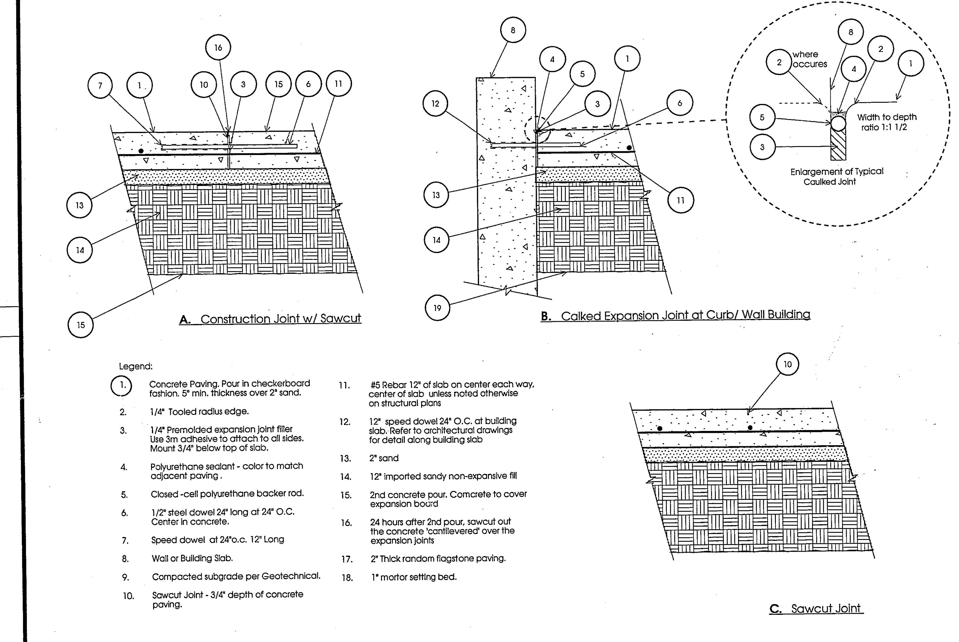
PAVING JOINTS
