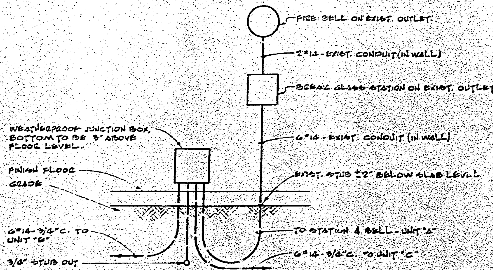
CONNECTIONS FOR F.A. AT UNIT 'A' NOT TO SCALE (SIMILAR FOR ALL BUILDINGS)
