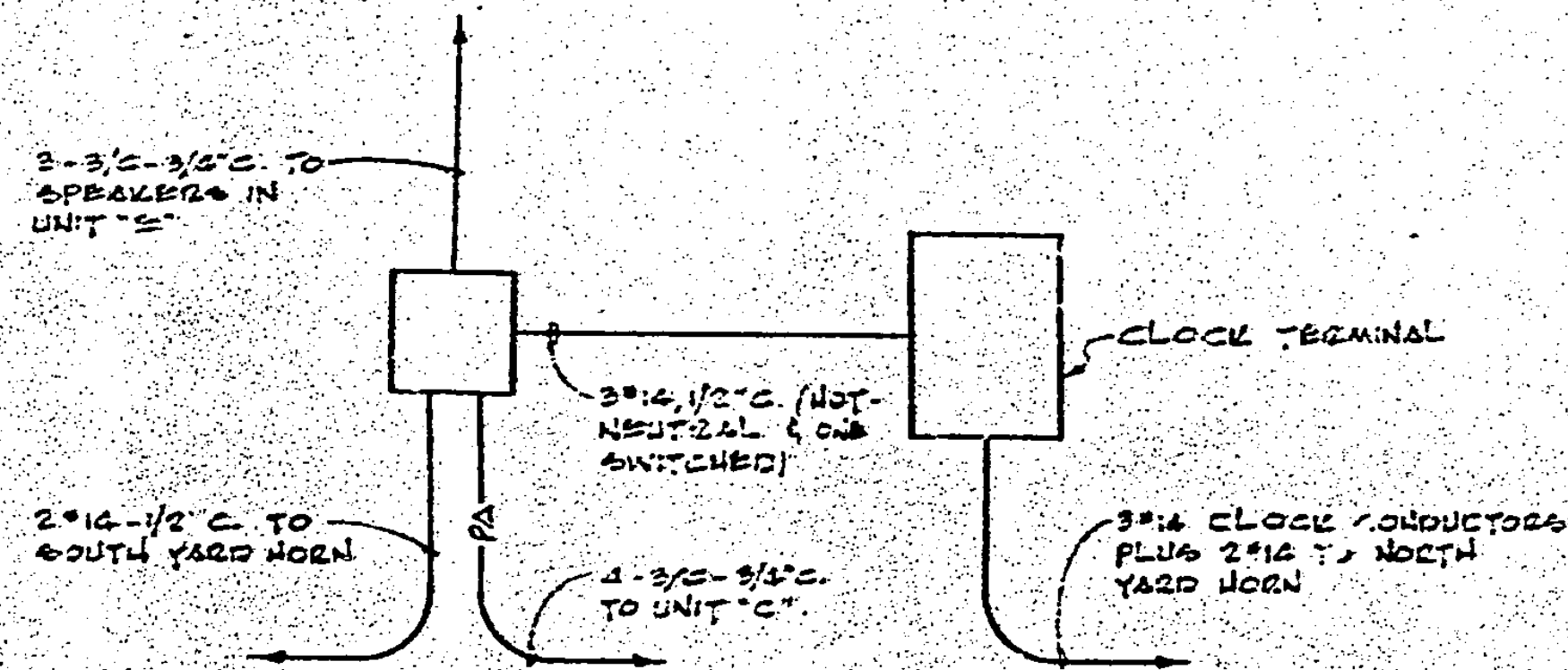
YARD HORN INTERCONNECTION AT MAIN PANEL CABINET NOT TO SCALE
