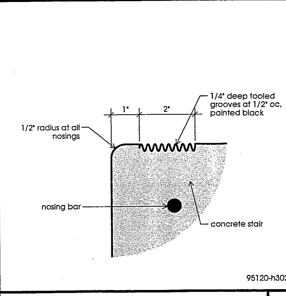
STAIR NOSING
