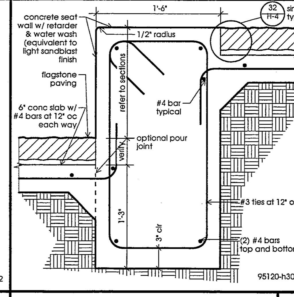
SEAT WALL
